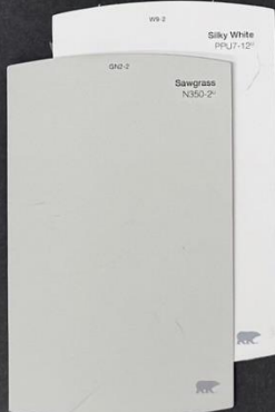
Scheme #209
