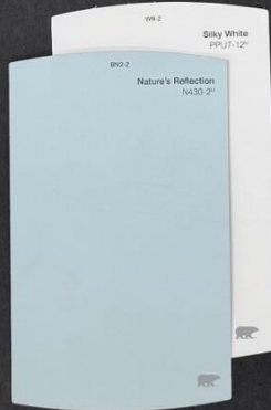
Scheme #210
